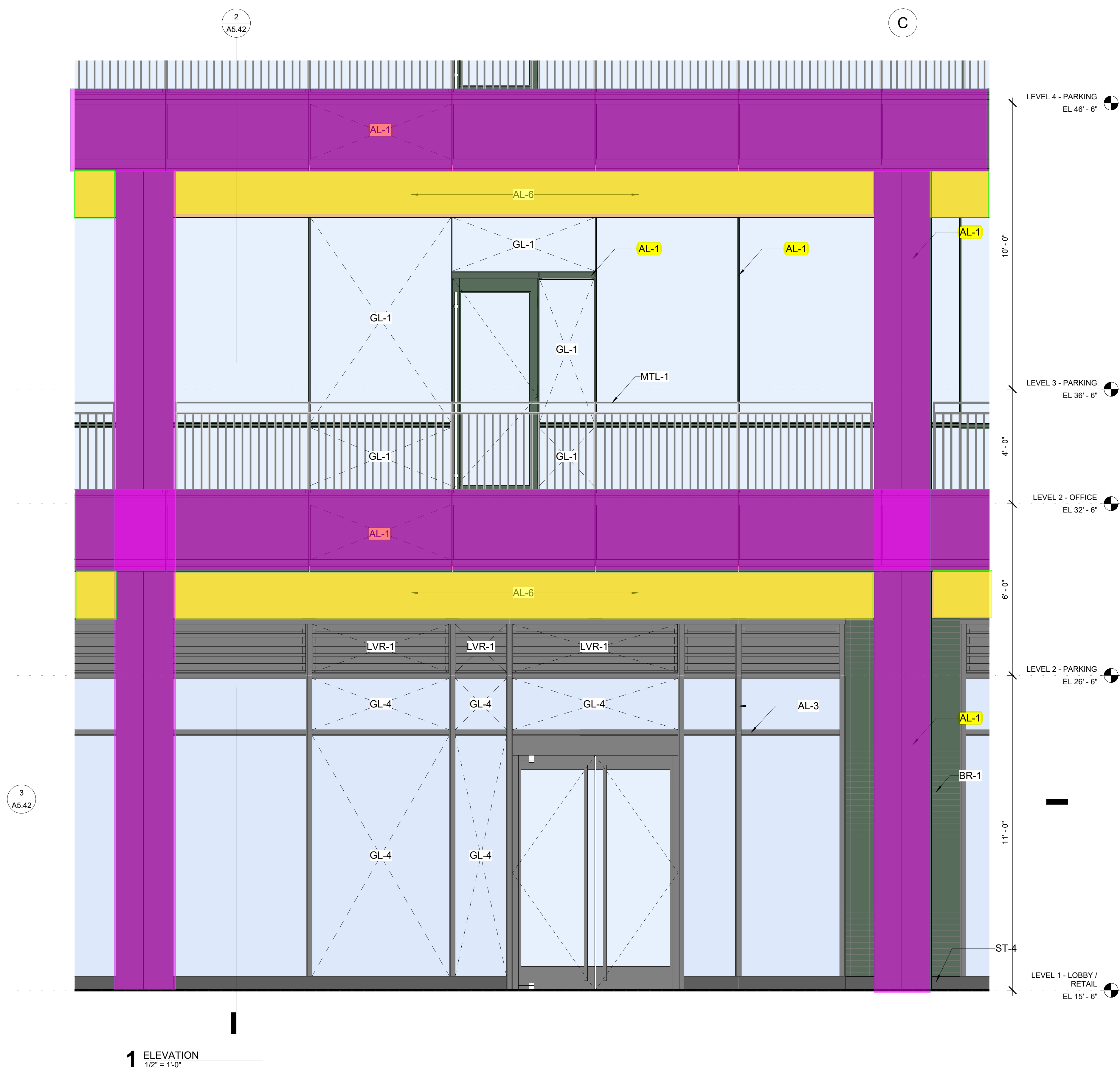
1 ELEVATION 1/2" = 1'-0"
