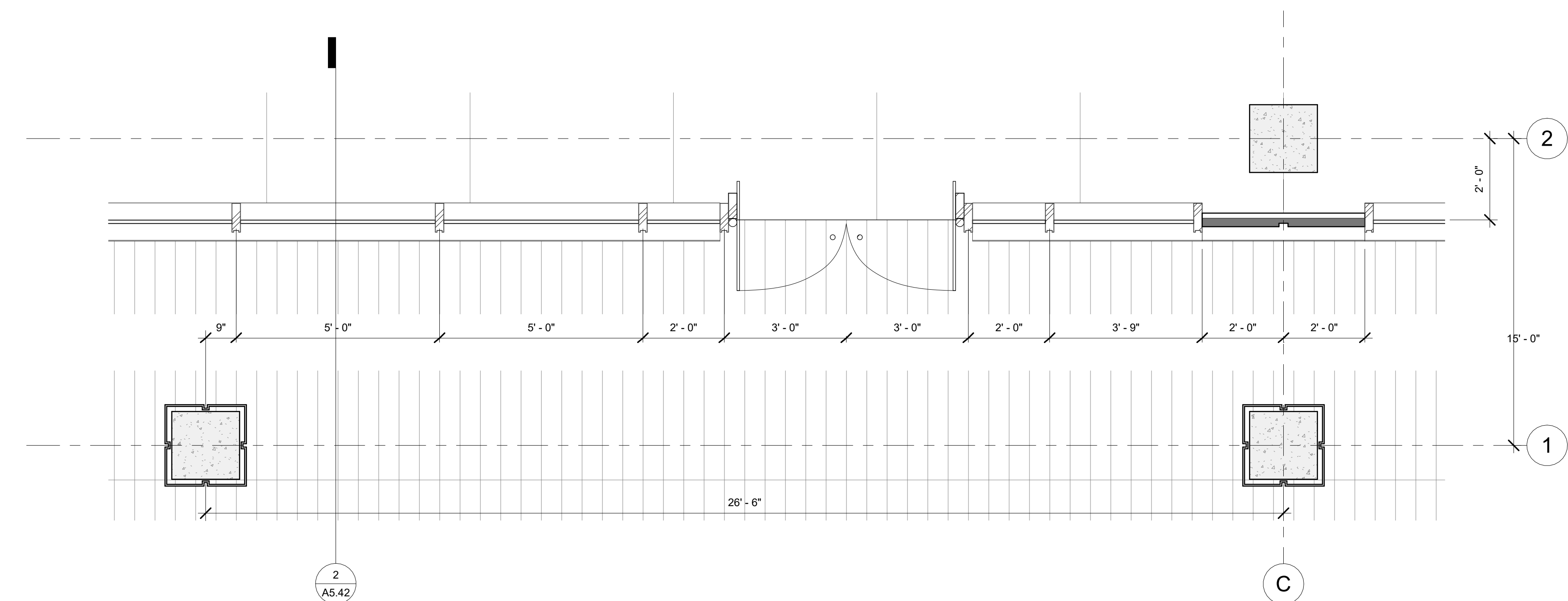
3 PLAN 1/2" = 1'-0"
